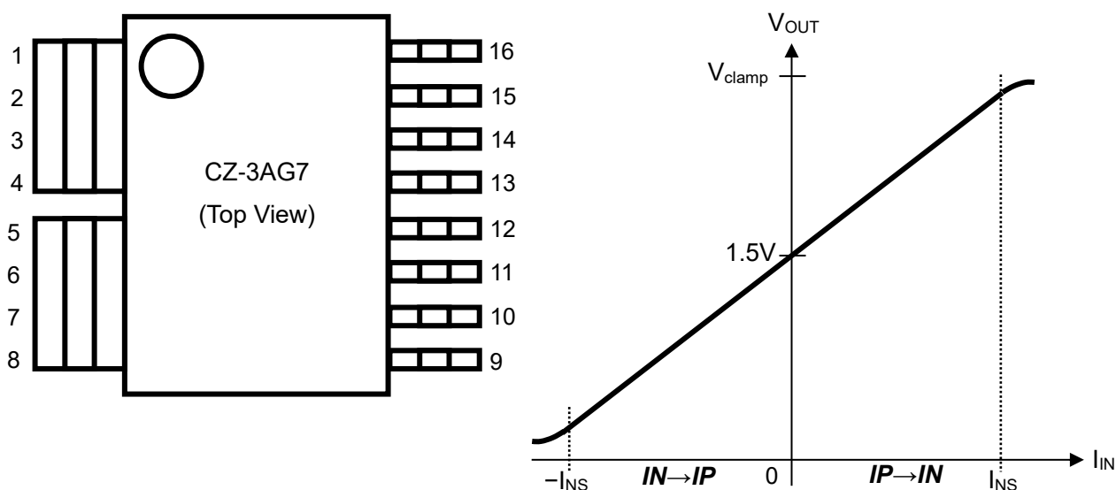
Figure 2. Pin configurations and typical output characteristics of CZ-3AG7
