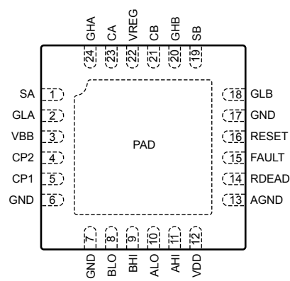
Pin-out Diagram
