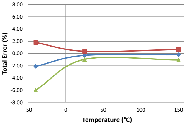
Total Error at I_{PR(max)} vs. Temperature
