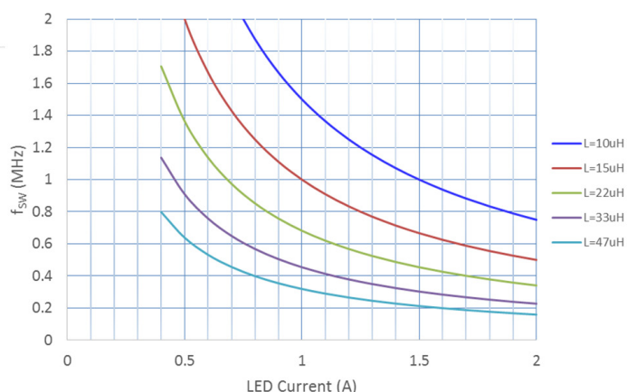
Figure 15: Minimum switching frequency vs. LED current, given different inductance used ( V_{IN} = 12 V, V_{OUT} = 6 V, ripple current = 20%)
