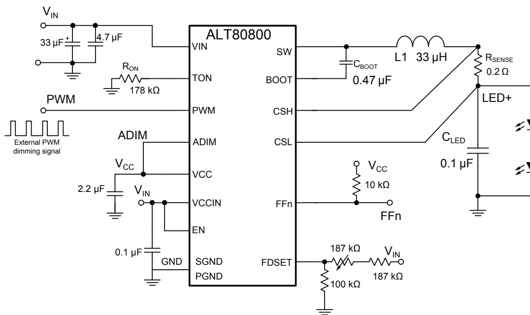
Figure 17: Application Circuit Example for ALT80800 (LED current = 1 A, 500 kHz)
