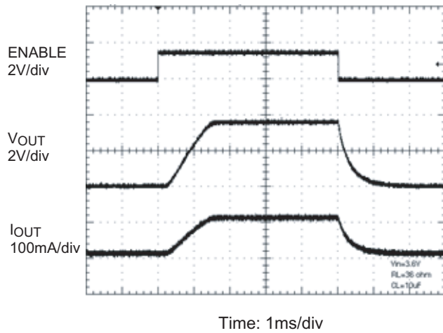
Turn-On/Turn-Off Timing
