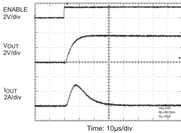
Turn-On Timing
