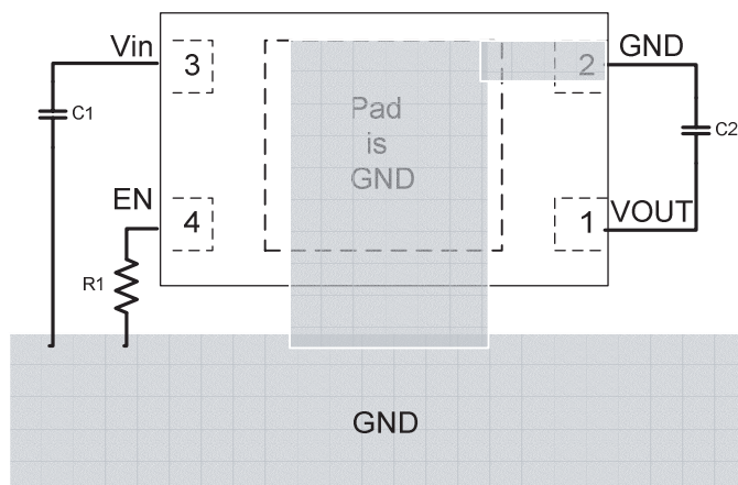
Figure 3. AOZ1321DI PCB Layout
