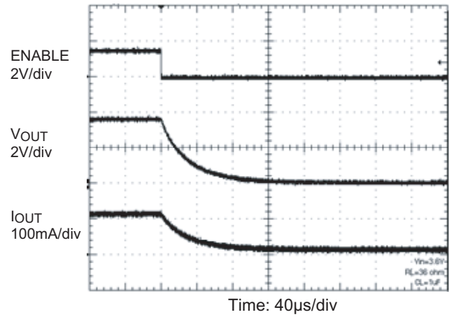
Turn-Off Timing
