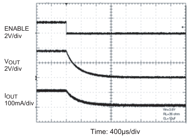
Turn-Off Timing
