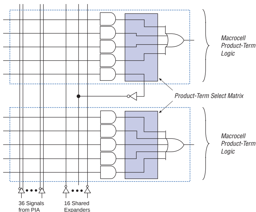
Figure 5. Shareable Expanders
