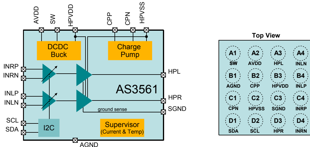
Figure 2. Pin Assignments (Top View)
