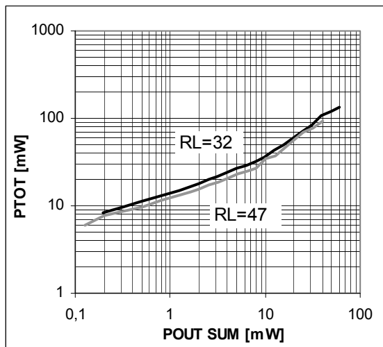
Figure 14. Total Power Consumption vrs. POUT for AVDD=5.0V
