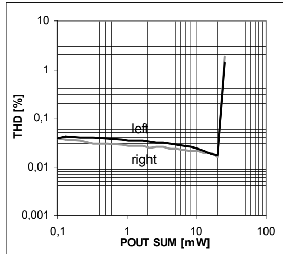
Figure 6. THD+N versus output power for AV_{DD}=3.6\text{ V} , R_L=47\Omega
