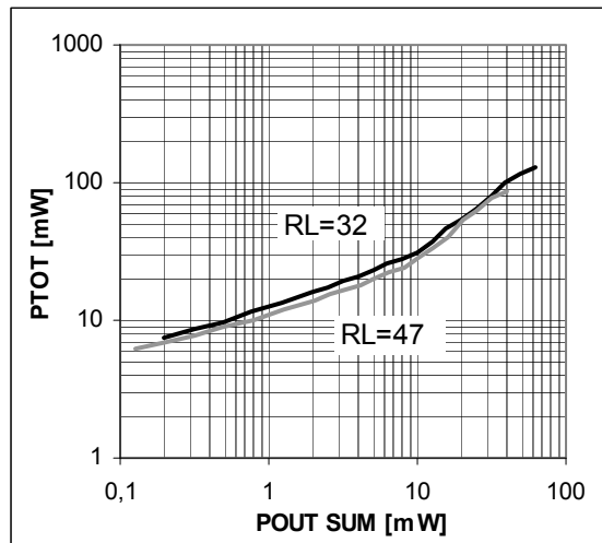
Figure 12. Total Power Consumption vrs. POUT for AVDD=3.6V
