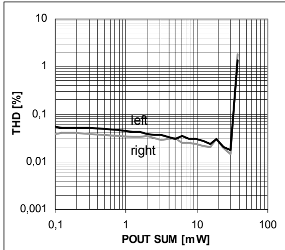
Figure 5. THD+N versus output power for AV_{DD}=3.6\text{ V} , R_L=32\Omega
