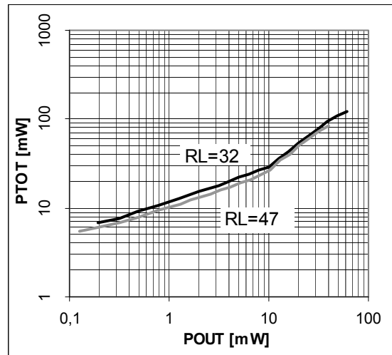
Figure 10. Total Power Consumption vrs. POUT for AVDD=2.5V
