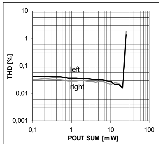
Figure 8. THD+N versus output power for AV_{DD}=5.0\text{ V} , R_L=47\Omega
