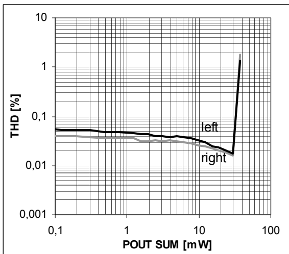
Figure 7. THD+N versus output power for AV_{DD}=5.0\text{ V} , R_L=32\Omega
