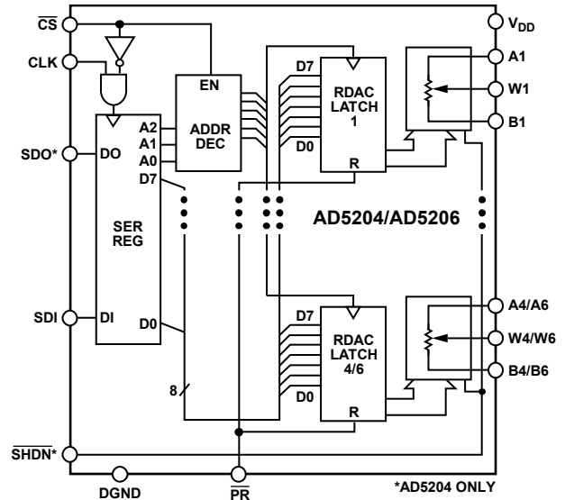
Figure 22. Block Diagram
