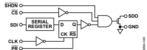
Figure 24. Detail SDO Output Schematic of the AD5204
