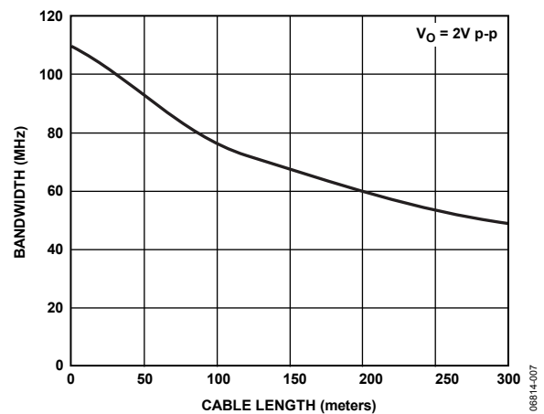
Figure 9. Equalized -3 dB Bandwidth vs. Cable Length
