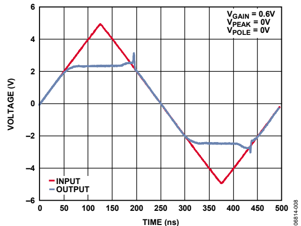
Figure 10. Overdrive Recovery
