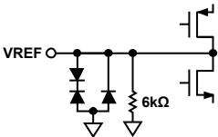
Figure 14. Equivalent VREF Circuit
