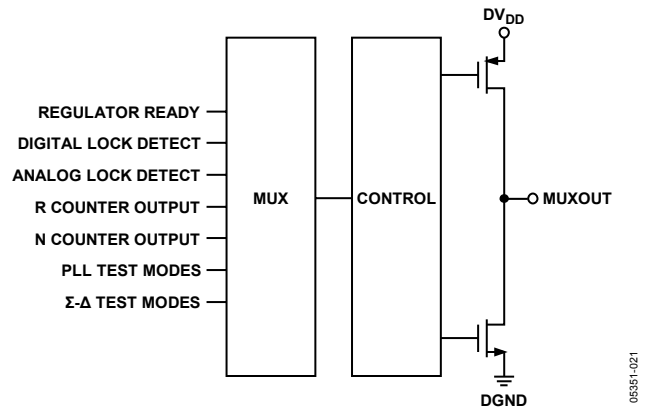
Figure 21. MUXOUT Circuit
