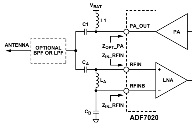
Figure 33. ADF7020 with Internal Rx/Tx Switch
