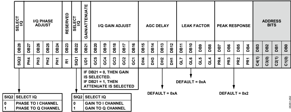
Figure 55. Register 10—AGC 2 Register
