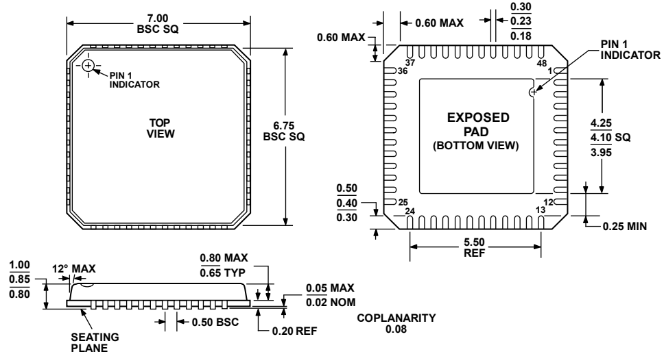
COMPLIANT TO JEDEC STANDARDS MO-220-VKGD-2 Figure 59. 48-Lead Lead Frame Chip Scale Package [LFCSP_VQ] 7 × 7 mm Body, Very Thin Quad (CP-48-3) Dimensions shown in millimeters
