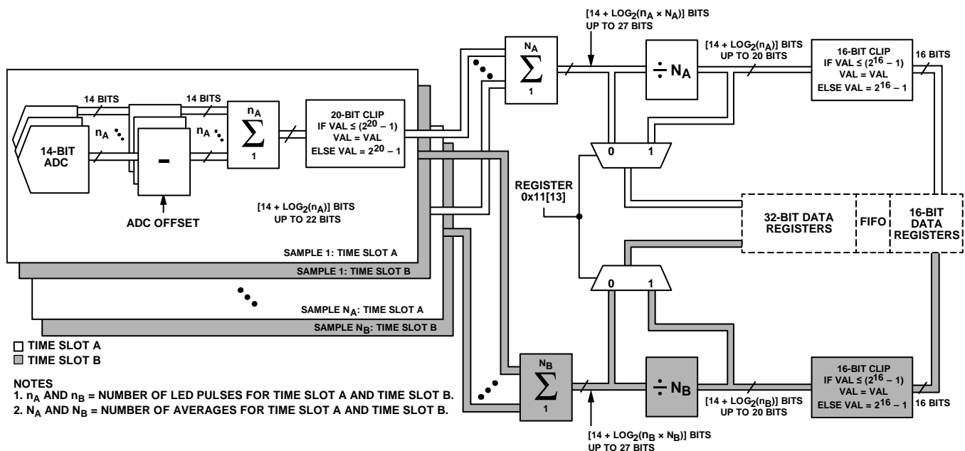
Figure 15. ADPD103 Datapath
