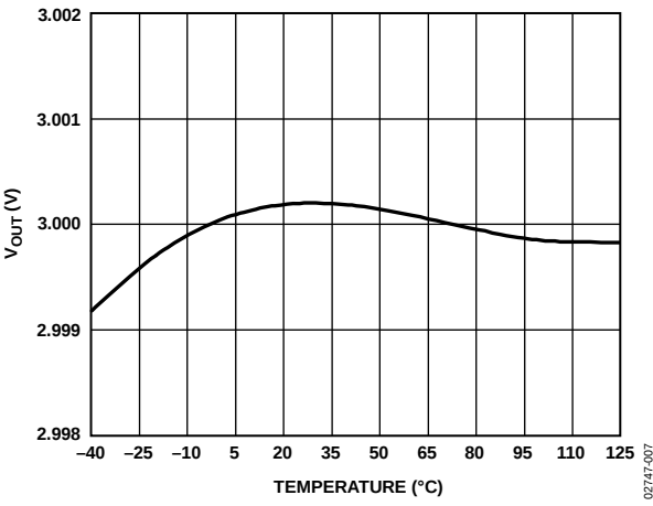
Figure 6. ADR06 Typical Output Voltage vs. Temperature
