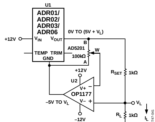
Figure 40. Programmable 0 mA to 5 mA Current Source
