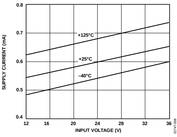
Figure 7. ADR01 Supply Current vs. Input Voltage
