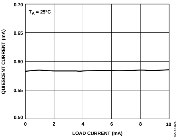
Figure 23. ADR01 Quiescent Current vs. Load Current
