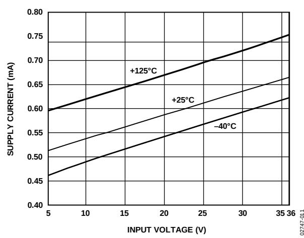
Figure 10. ADR06 Supply Current vs. Input Voltage
