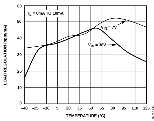
Figure 13. ADR03 Load Regulation vs. Temperature
