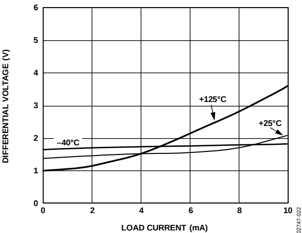
Figure 21. ADR03 Dropout Voltage vs. Load Current
