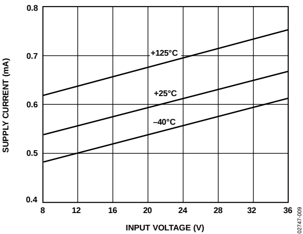
Figure 8. ADR02 Supply Current vs. Input Voltage
