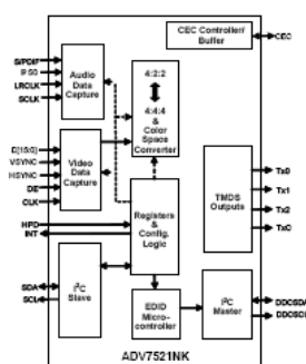
Functional Block Diagram for ADV7521NK
