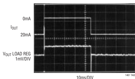
LT1461-2.5 Load Regulation, P DISS = 200mW
