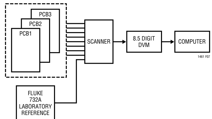
Figure 7. Long-Term Drift Measurement Setup
