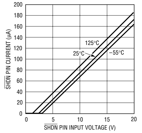
SHDN Pin Current vs SHDN Input Voltage
