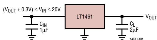
Basic Connection
