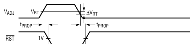
Comparator Mode UVLO Timing
