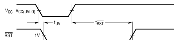
Normal UVLO Timing
