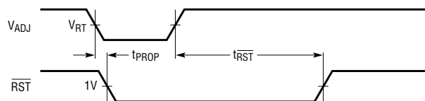
Normal Negative Polarity Input Timing
