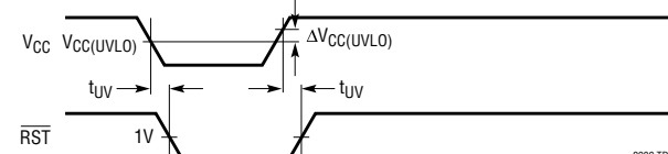
Comparator Mode UVLO Timing
