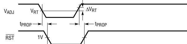
Comparator Mode Negative Polarity Input Timing
