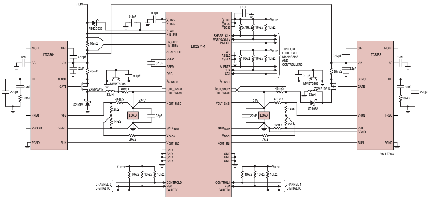
LTC2971-1 +48V to ±24V with Wide Margining Range
