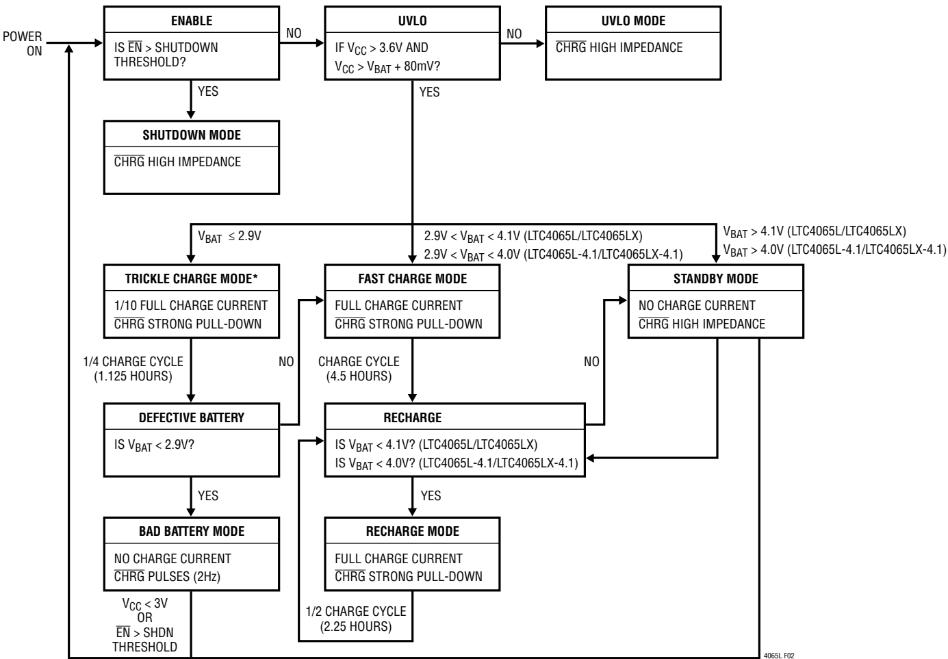
Figure 2. State Diagram of LTC4065L Operation
