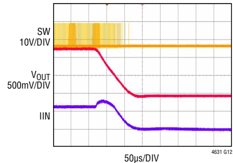
Single Phase Short Circuit Protection with 10A
