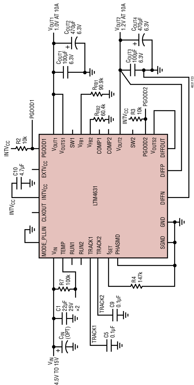
Figure 23. Typical 4.5V IN to 15V IN , 1.0V and 1.2V at 10A Outputs
