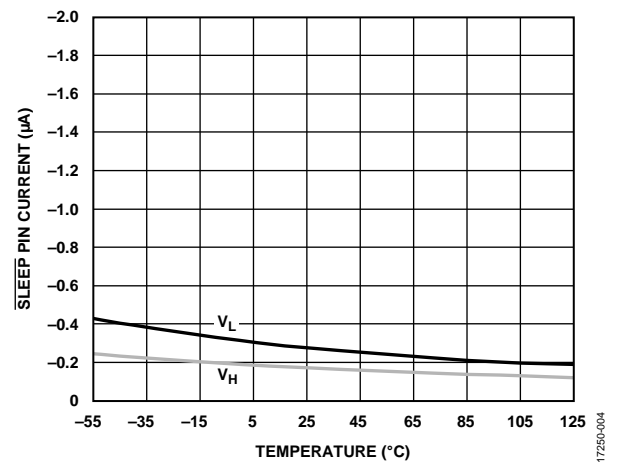
Figure 4. \overline{SLEEP} Pin Current vs. Temperature
