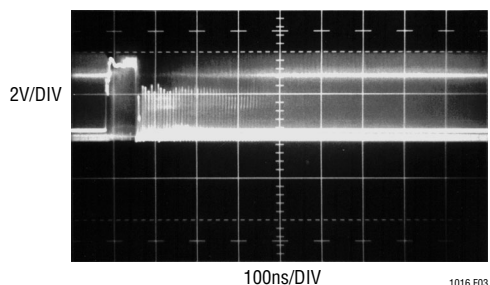
Figure 3. Unbypassed LT1016 Response
