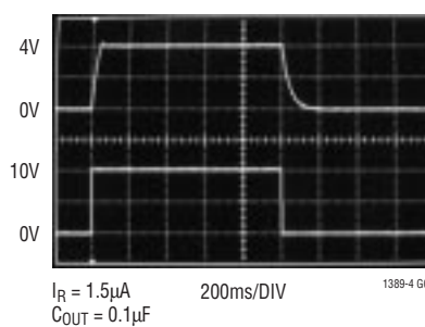
Response Time
