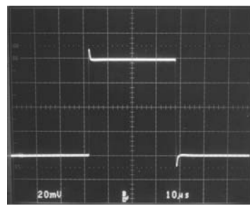
Small-Signal Response
