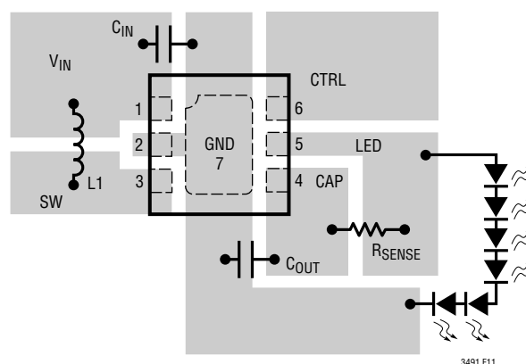
(B) DFN PACKAGE
