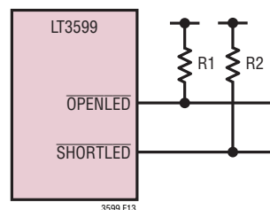
Figure 12. \overline{\text{OPENLED}} and \overline{\text{SHORTLED}} Connection
