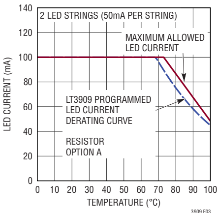
Figure 3. LED Current Derating vs LED Ambient Temperature
