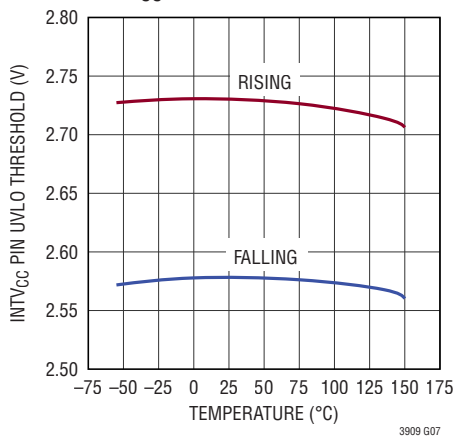
INTV CC Pin UVLO Threshold
