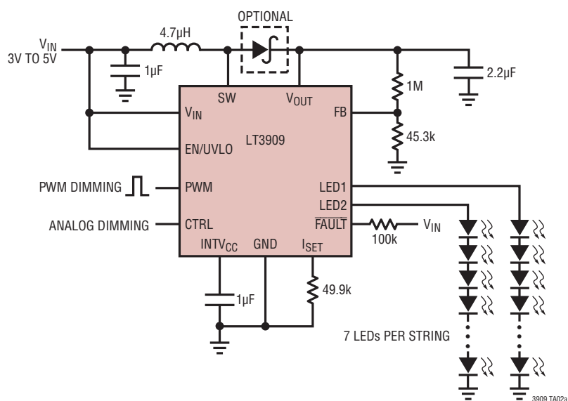
2-String × 20mA Driver for Seven White LEDs/String
