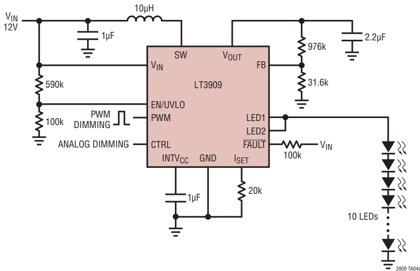
12V Input, 1 String × 100mA Driver for Ten White LEDs
