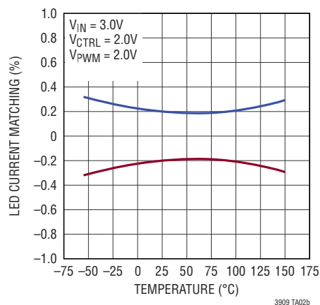
LED Current Matching (Normalized to 2-String Average)
