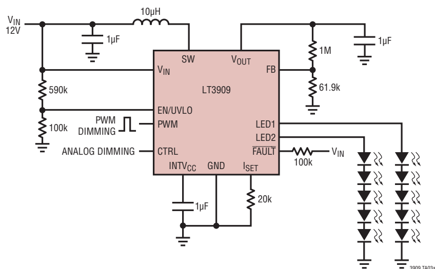
12V Input, 2-String × 50mA Driver for Five White LEDs/String
