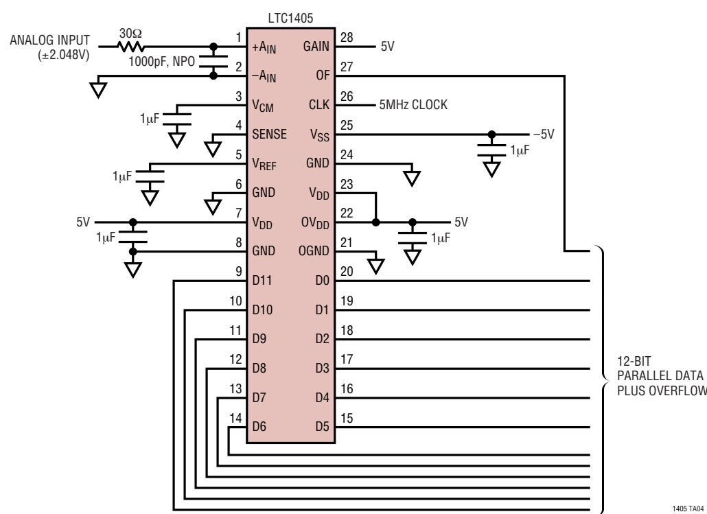
Dual Supply, 5Msps, 12-Bit ADC with 71.3dB SINAD
