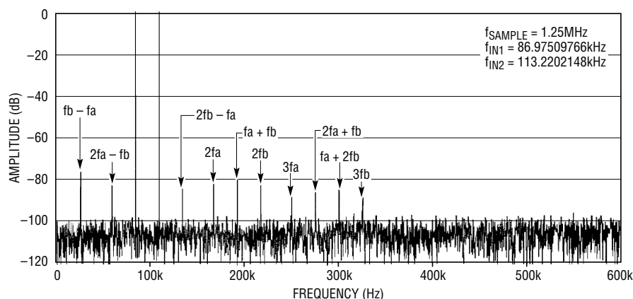
Figure 5. Intermodulation Distortion Plot
