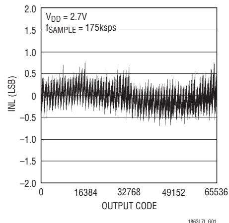
Integral Nonlinearity vs Output Code (LTC1867L)
