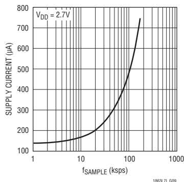
Figure 5. Supply Current vs f_{\text{SAMPLE}}
