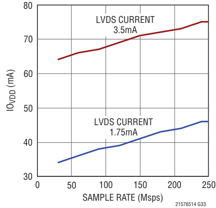
LTC2156-14: I_{QVDD} vs Sample Rate, 15MHz Sine Wave Input, -1dBFS
