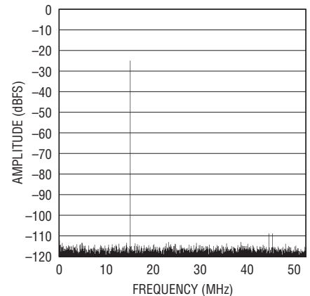
LTC2207-14: 64K Point FFT, f_{IN} = 15.1\text{MHz} , -25\text{dBFS} , PGA = 0, RAND "On", Dither "Off"
