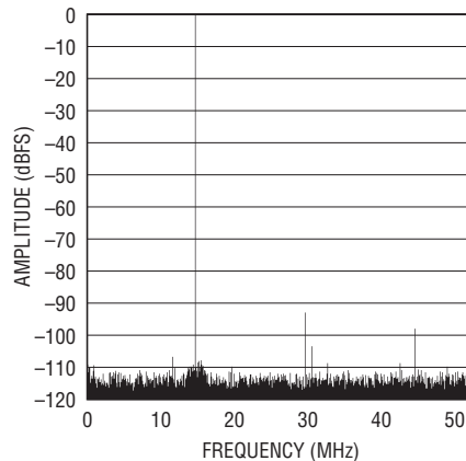
LTC2207-14: 32K Point FFT, f_{IN} = 14.86\text{MHz} , -1\text{dBFS} , PGA = 0, RAND "On", Dither "Off"
