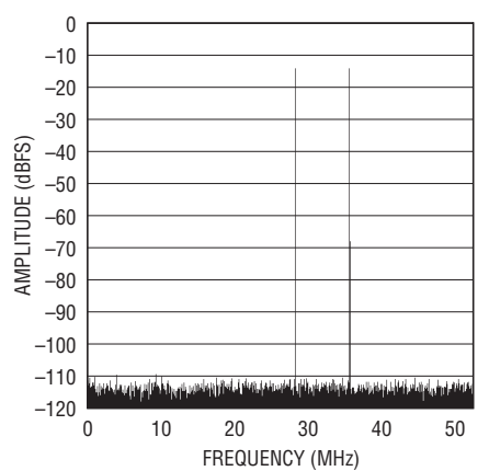
LTC2207-14: 32K Point 2-Tone FFT, f_{IN} = 69.2\text{MHz} and 76.5\text{MHz} , -15\text{dBFS} , \text{PGA} = 0 , \text{RAND} "On", Dither "Off"
