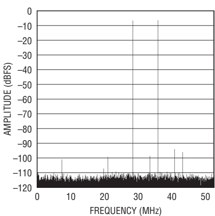
LTC2207-14: 32K Point 2-Tone FFT, f_{IN} = 69.2\text{MHz} and 76.5\text{MHz} , -7\text{dBFS} , \text{PGA} = 0 , \text{RAND} "On", Dither "Off"
