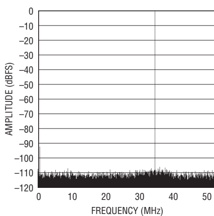
LTC2207-14: 32K Point FFT, f_{IN} = 70.24\text{MHz} , -1\text{dBFS} , \text{PGA} = 1 , \text{RAND} "On", Dither "Off"
