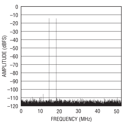
LTC2207-14: 32K Point 2-Tone FFT, f_{IN} = 14.87\text{MHz} and 18.56\text{MHz} , -15\text{dBFS} , \text{PGA} = 0 , \text{RAND} "On", Dither "Off"
