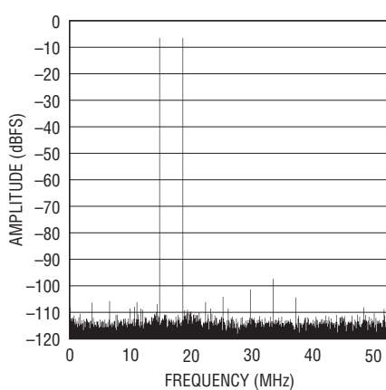
LTC2207-14: 32K Point 2-Tone FFT, f_{IN} = 14.87\text{MHz} and 18.56\text{MHz} , -7\text{dBFS} , \text{PGA} = 0 , \text{RAND} "On", Dither "Off"
