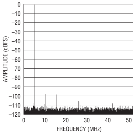
LTC2207-14: 32K Point FFT, f_{IN} = 5.23\text{MHz} , -1\text{dBFS} , PGA = 0, RAND "On", Dither "Off"
