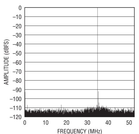
LTC2207-14: 32K Point FFT, f_{IN} = 70.24\text{MHz} , -1\text{dBFS} , \text{PGA} = 0 , \text{RAND} "On", Dither "Off"
