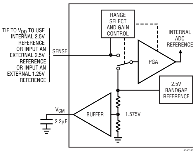
Figure 6. Reference Circuit
