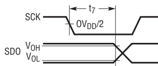
Figure 3. SDO Data Valid Hold After SCK↓
