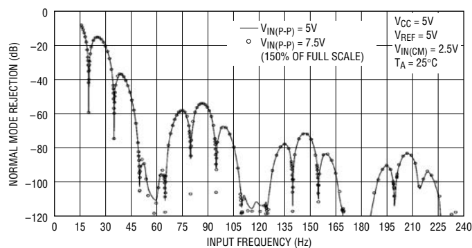
Figure 18. Measure Input Normal Mode Rejection vs Input Frequency with Input Perturbation of 150% (60Hz Notch)
