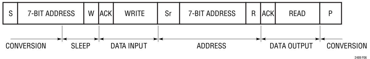
Figure 6. Write, Read, Start Conversion
