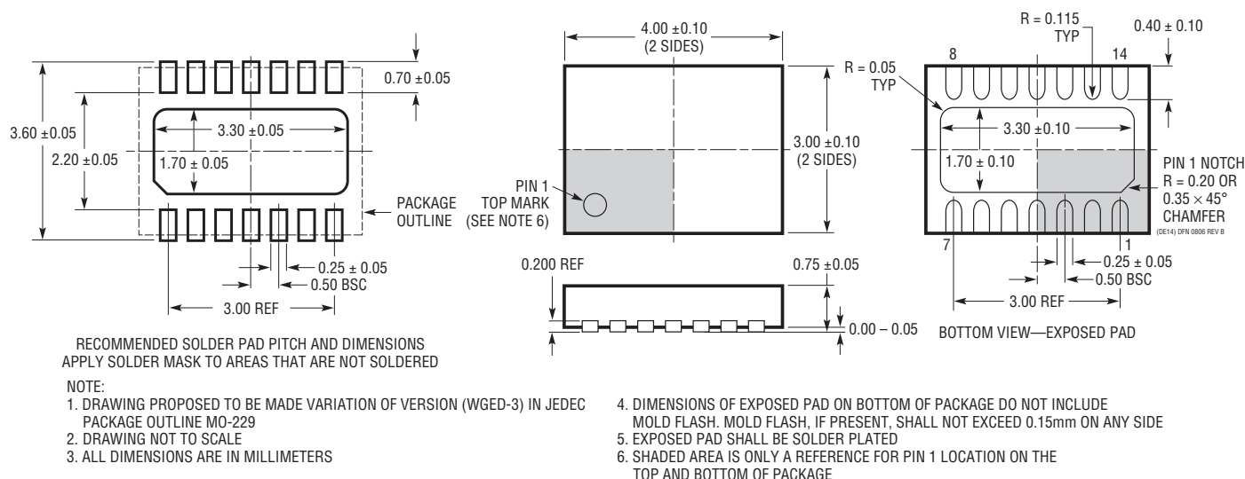
DE Package 14-Lead Plastic DFN (4mm \times 3mm) (Reference LTC DWG # 05-08-1708 Rev B)
