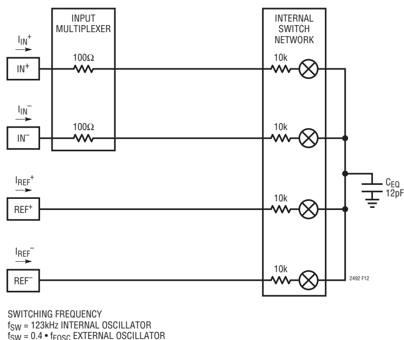
Figure 12. LTC2492 Equivalent Analog Input Circuit
