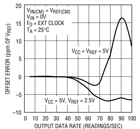
Figure 25. Offset Error vs Output Data Rate and Temperature
