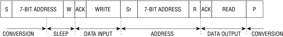
Figure 6. Write, Read, Start Conversion
