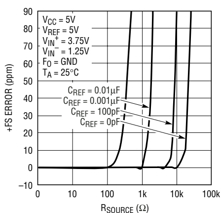
Figure 11. +FS Error vs R_{\text{SOURCE}} at V_{\text{REF}} (Small C_{\text{REF}} )
