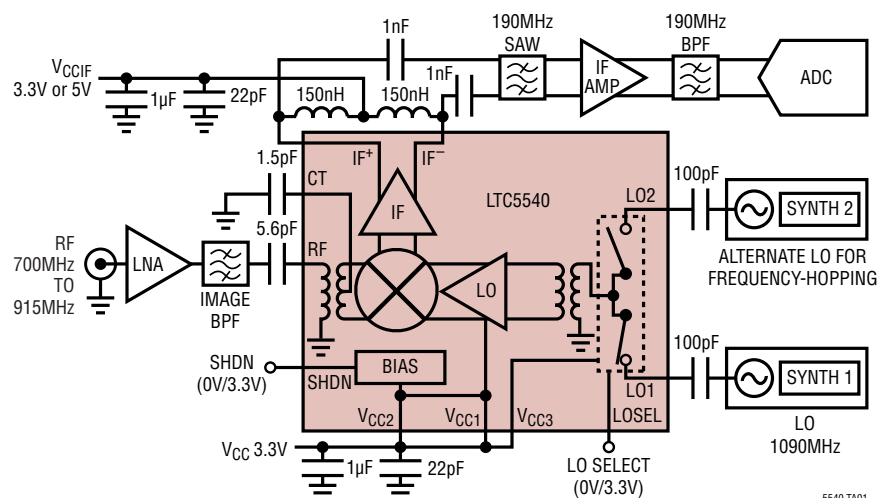
Wideband Receiver
