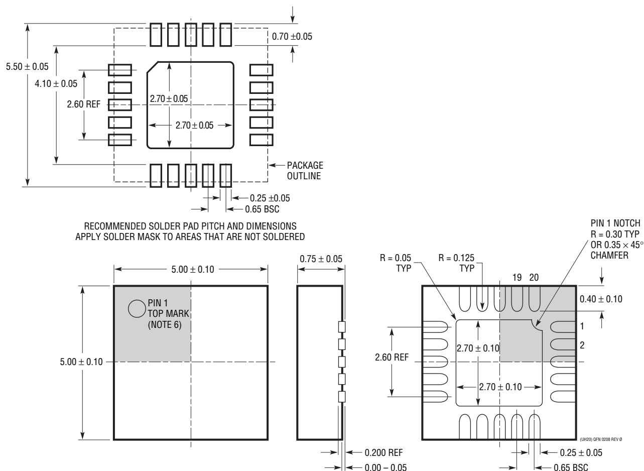
BOTTOM VIEW—EXPOSED PAD
