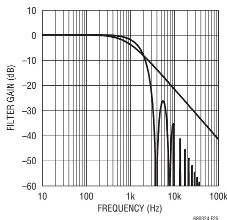
Figure 25. Noise Filtering of the LTC6803-4 ADC
