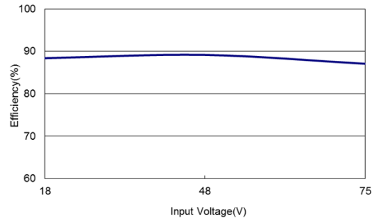
Figure 74: ERM01H36 Efficiency Versus Input Voltage Curve Vin = 18 to 75Vdc Load: Io = 0.833A
