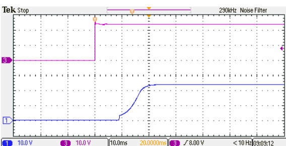
Figure 29: ERM01H18 Output Voltage Startup Characteristic by Vin Vin = 24Vdc Load: Io = 0.833A Ch1: Vin Ch3: Vo
