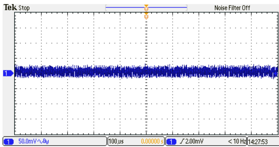
Figure 75: ERM01H36 Ripple and Noise Measurement Vin = 48Vdc Load: Io = 0.833A Ch 1: Vo
