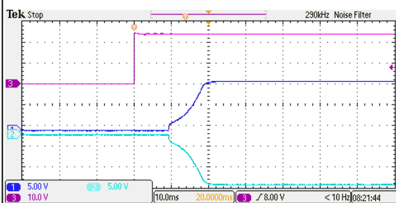
Figure 37: ERM01BB18 Output Voltage Startup Characteristic by Vin Vin = 24Vdc Load: Io = \pm 0.833A Ch1: Vo1 Ch2: Vo2 Ch3: Vin
