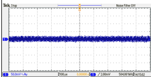
Figure 67: ERM01C36 Ripple and Noise Measurement Vin = 48Vdc Load: Io = 1.33A Ch 1: Vo
