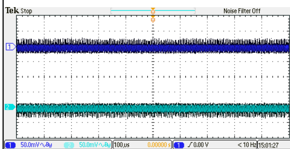
Figure 83: ERM01BB36 Ripple and Noise Measurement Vin = 48Vdc Load: Io = \pm 0.833A Ch 1: Vo
