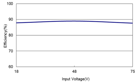
Figure 58: ERM01B36 Efficiency Versus Input Voltage Curve Vin = 18 to 75Vdc Load: Io = 1.67A
