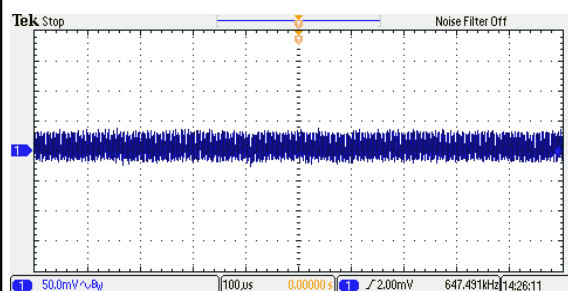
Figure 27: ERM01H18 Ripple and Noise Measurement Vin = 24Vdc Load: Io = 0.833A Ch 1: Vo
