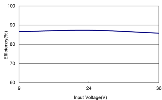
Figure 34: ERM01BB18 Efficiency Versus Input Voltage Curve Vin = 9 to 36Vdc Load: Io = 0 to \pm 0.833A
