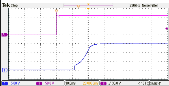
Figure 117: ERM01C110 Output Voltage Startup Characteristic by V_{in} V_{in} = 110Vdc Load: I_o = 1.33A Ch1: V_o Ch3: V_{in}
