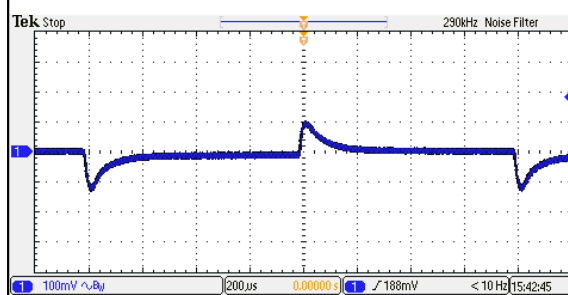
Figure 124: ERM01H36 Transient Response Vin = 110Vdc Load: Io = 100% to 75% load change Ch 1: Vo
