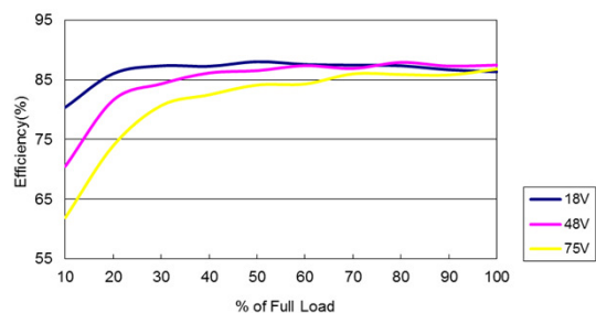
Figure 49: ERM04A36 Efficiency Versus Output Current Curve Vin = 18 to 75Vdc Load: Io = 0 to 4A
