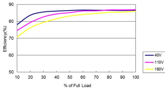
Figure 137: ERM01CC110 Efficiency Versus Output Current Curve Vin = 40 to 160Vdc Load: Io = 0 to \pm 0.667A
