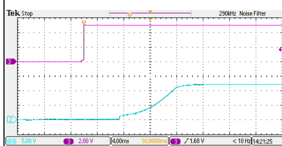
Figure 14: ERM01B18 Output Voltage Startup Characteristic by On/Off Vin = 24Vdc Load: I_o = 1.67A Ch2: Vo Ch3: Vin
