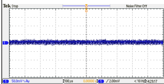
Figure 123: ERM01H36 Ripple and Noise Measurement Vin = 110Vdc Load: Io = 0.833A Ch 1: Vo
