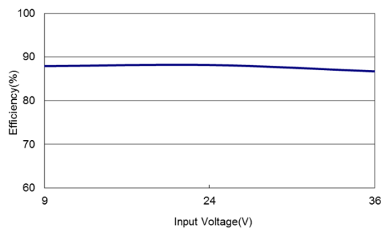
Figure 10: ERM01B18 Efficiency Versus Input Voltage Curve Vin = 9 to 36Vdc Load: I_o = 1.67A
