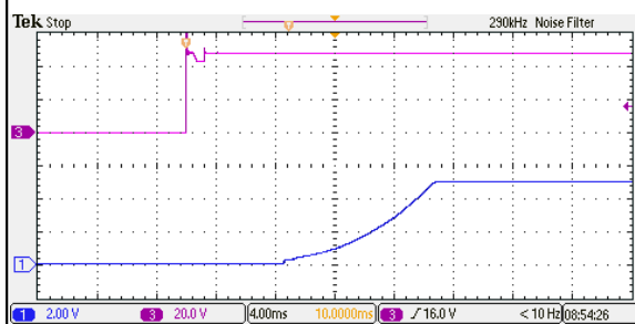
Figure 53: ERM04A36 Output Voltage Startup Characteristic by Vin Vin = 48Vdc Load: Io = 4A Ch1: Vo Ch3: Vin
