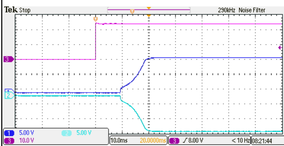
Figure 45: ERM01CC18 Output Voltage Startup Characteristic by Vin Vin = 24Vdc Load: Io = \pm 0.667A Ch1: Vo1 Ch2: Vo2 Ch3: Vin
