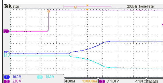
Figure 94: ERM01CC36 Output Voltage Startup Characteristic by On/Off Vin = 48Vdc Load: Io = \pm 0.667A Ch1: Vo1 Ch2:Vo2 Ch3: Vin
