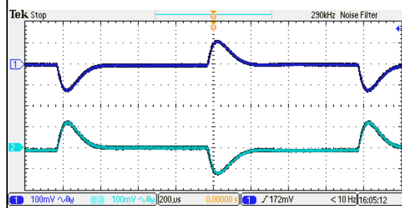
Figure 132: ERM01BB110 Transient Response Vin = 110Vdc Load: I_o = 100\% to 75\% load change Ch1: Vo1 Ch2: Vo2
