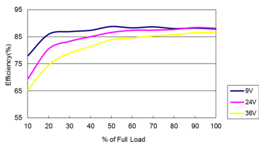
Figure 25: ERM01H18 Efficiency Versus Output Current Curve Vin = 9 to 36Vdc Load: Io = 0 to 0.833A
