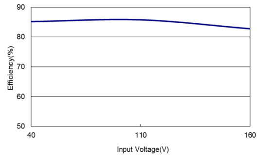
Figure 98: ERM04A110 Efficiency Versus Input Voltage Curve Vin = 40 to 160Vdc Load: Io = 4A
