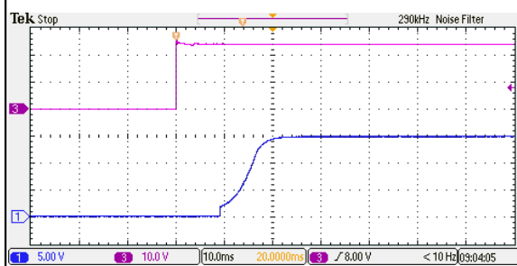
Figure 21: ERM01C18 Output Voltage Startup Characteristic by Vin Vin = 24Vdc Load: Io = 1.33A Ch1: Vin Ch3: Vo
