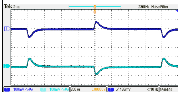
Figure 84: ERM01BB36 Transient Response Vin = 48Vdc Load: Io = 100% to 75% load change Ch 1: Vo
