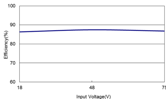
Figure 50: ERM04A36 Efficiency Versus Input Voltage Curve Vin = 18 to 75Vdc Load: Io = 4A
