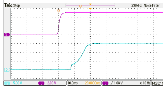
Figure 118: ERM01C110 Output Voltage Startup Characteristic by On/Off V_{in} = 110Vdc Load: I_o = 1.33A Ch2: V_o Ch3: V_{in}
