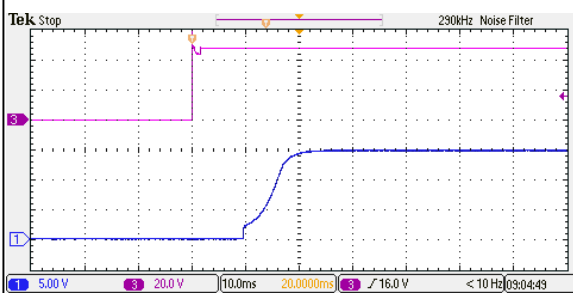
Figure 69: ERM01C36 Output Voltage Startup Characteristic by Vin Vin = 48Vdc Load: Io = 1.33A Ch1: Vo Ch3: Vin
