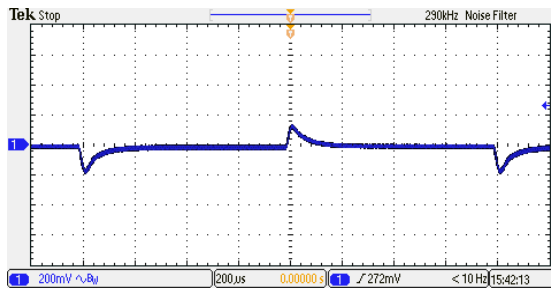
Figure 76: ERM01H36 Transient Response Vin = 48Vdc Load: Io = 100% to 75% load change Ch 1: Vo
