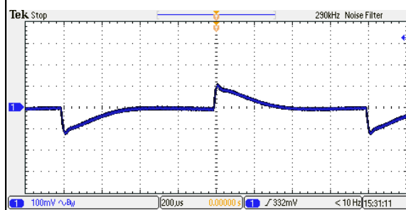
Figure 52: ERM04A36 Transient Response Vin = 48Vdc Load: Io = 100% to 75% load change Ch 1: Vo
