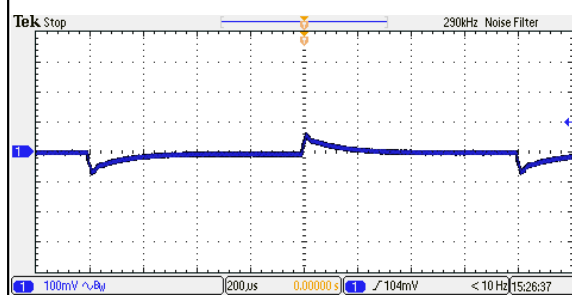
Figure 20: ERM01C18 Transient Response Vin = 24Vdc Load: Io = 100% to 75% load change Ch 1: Vo
