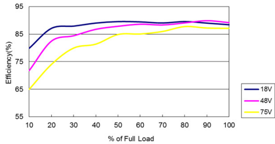
Figure 73: ERM01H36 Efficiency Versus Output Current Curve Vin = 18 to 75Vdc Load: Io = 0 to 0.833A
