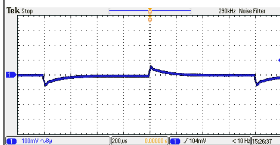
Figure 4: ERM04A18 Transient Response Vin = 24Vdc Load: Io = 100% to 75% load change Ch 1: Vo
