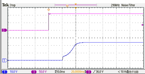
Figure 125: ERM01H36 Output Voltage Startup Characteristic by Vin Vin = 110Vdc Load: Io = 0.833A Ch1: Vo Ch3: Vin
