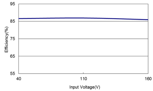
Figure 138: ERM01CC110 Efficiency Versus Input Voltage Curve Vin = 40 to 160Vdc Load: Io = \pm 0.667A
