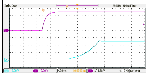
Figure 102: ERM04A110 Output Voltage Startup Characteristic by On/Off Vin = 110Vdc Load: Io = 4A Ch2: Vo Ch3: Vin
