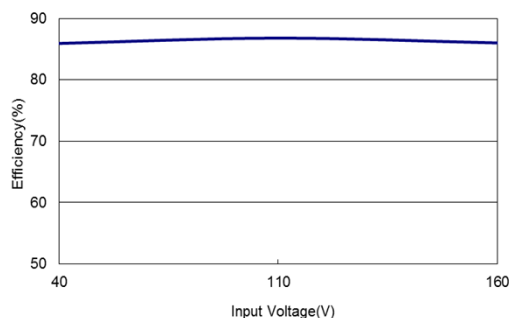
Figure 106: ERM01B110 Efficiency Versus Input Voltage Curve Vin = 40 to 160Vdc Load: I_o = 1.67A
