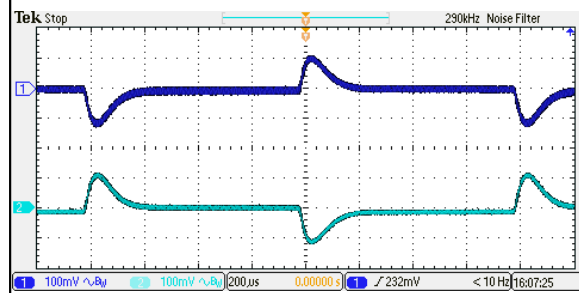
Figure 140: ERM01CC110 Transient Response Vin = 110Vdc Load: Io = 100% to 75% load change Ch 1: Vo1 Ch 2: Vo2
