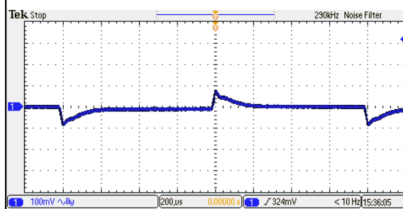
Figure 708: ERM01B110 Transient Response Vin = 110Vdc Load: I_o = 100\% to 75% load change Ch 1: Vo
