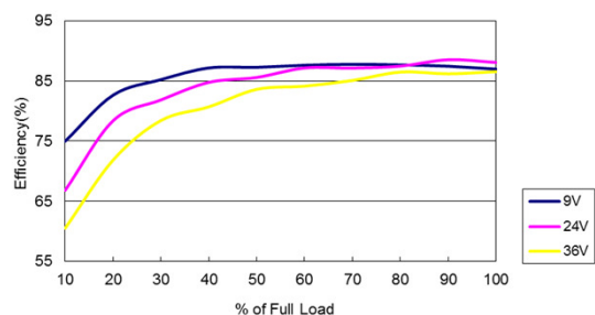
Figure 1: ERM04A18 Efficiency Versus Output Current Curve Vin = 9 to 36Vdc Load: Io = 0 to 4A
