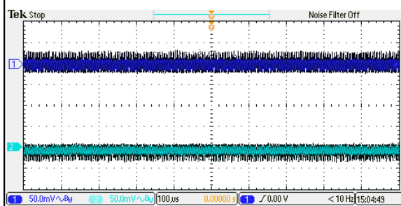
Figure 91: ERM01CC36 Ripple and Noise Measurement Vin = 48Vdc Load: Io = \pm 0.667A Ch 1: Vo1 Ch 2: Vo2
