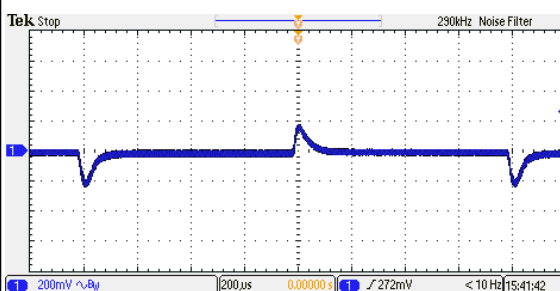
Figure 28: ERM01H18 Transient Response Vin = 24Vdc Load: Io = 100% to 75% load change Ch 1: Vo
