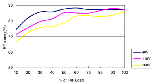
Figure 121: ERM01H36 Efficiency Versus Output Current Curve Vin = 40 to 160Vdc Load: Io = 0 to 0.833A
