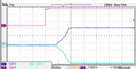
Figure 85: ERM01BB36 Output Voltage Startup Characteristic by Vin Vin = 48Vdc Load: Io = \pm 0.833A Ch1: Vo1 Ch2: Vo2 Ch3: Vin
