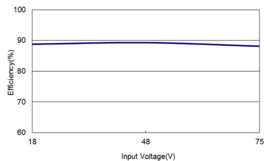
Figure 90: ERM01CC36 Efficiency Versus Input Voltage Curve Vin = 18 to 75Vdc Load: Io = \pm 0.667A
