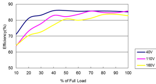
Figure 97: ERM04A110 Efficiency Versus Output Current Curve Vin = 40 to 160Vdc Load: Io = 0 to 4A
