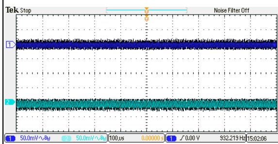
Figure 131: ERM01BB110 Ripple and Noise Measurement Vin = 110Vdc Load: I_o = \pm 0.833A Ch1: Vo1 Ch2: Vo2
