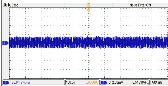
Figure 59: ERM01B36 Ripple and Noise Measurement Vin = 48Vdc Load: Io = 1.67A Ch 1: Vo
