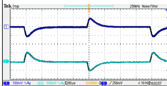
Figure 36: ERM01BB18 Transient Response Vin = 24Vdc Vin = 24Vdc Load: Io = 100% to 75% load change Ch 1: Vo1 Ch2: Vo2
