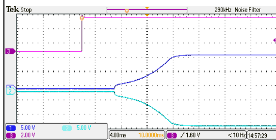
Figure 86: ERM01BB36 Output Voltage Startup Characteristic by On/Off Vin = 48Vdc Load: Io = \pm 0.833A Ch1: Vo1 Ch2: Vo2 Ch3: Vin
