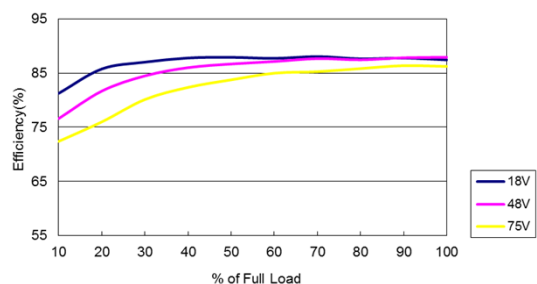
Figure 81: ERM01BB36 Efficiency Versus Output Current Curve Vin = 18 to 75Vdc Load: Io = 0 to \pm 0.833A
