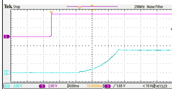
Figure 6: ERM04A18 Output Voltage Startup Characteristic by On/Off Vin = 24Vdc Load: Io = 4A Ch2: Vo Ch3: Vin
