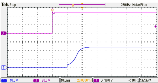
Figure 77: ERM01H36 Output Voltage Startup Characteristic by Vin Vin = 48Vdc Load: Io = 0.833A Ch1: Vo Ch3: Vin
