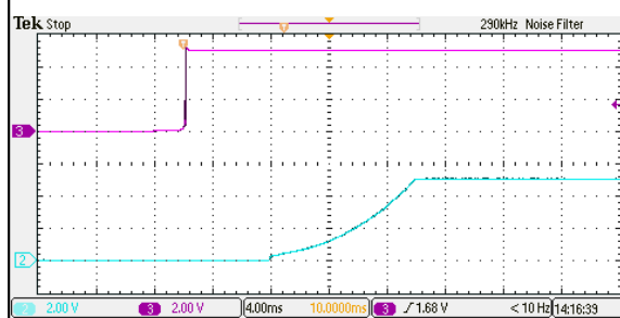
Figure 54: ERM04A36 Output Voltage Startup Characteristic by On/Off Vin = 48Vdc Load: Io = 4A Ch2: Vo Ch3: Vin
