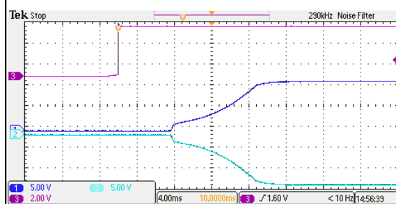
Figure 38: ERM01BB18 Output Voltage Startup Characteristic by On/Off Vin = 24Vdc Load: Io = \pm 0.833A Ch1: Vo1 Ch2: Vo2 Ch3: Vin
