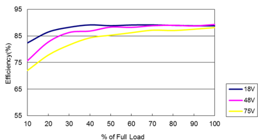
Figure 89: ERM01CC36 Efficiency Versus Output Current Curve Vin = 18 to 75Vdc Load: Io = 0 to \pm 0.667A
