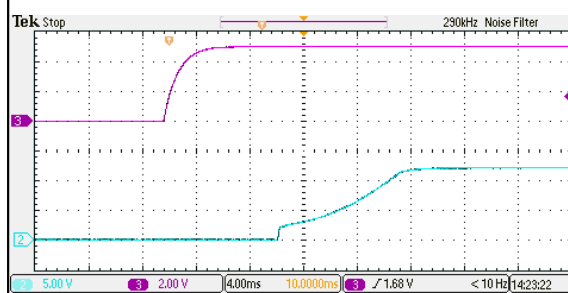
Figure 110: ERM01B110 Output Voltage Startup Characteristic by On/Off Vin = 110Vdc Load: I_o = 1.67A Ch2: Vo Ch3: Vin
