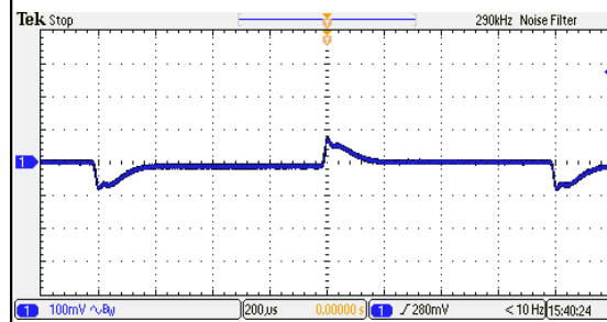
Figure 116: ERM01C110 Transient Response V_{in} = 110Vdc Load: I_o = 100\% to 75% load change Ch 1: V_o
