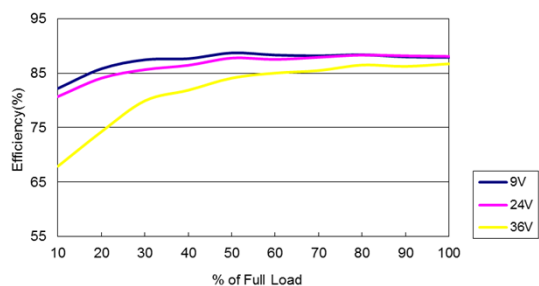
Figure 9: ERM01B18 Efficiency Versus Output Current Curve Vin = 9 to 36Vdc Load: I_o = 0 to 1.67A
