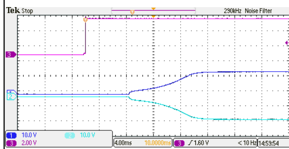
Figure 46: ERM01CC18 Output Voltage Startup Characteristic by On/Off Vin = 24Vdc Load: Io = \pm 0.667A Ch1: Vo1 Ch2: Vo2 Ch3: Vin
