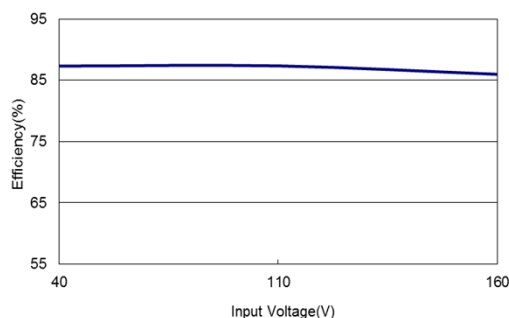
Figure 122: ERM01H36 Efficiency Versus Input Voltage Curve Vin = 40 to 160Vdc Load: Io = 0.833A
