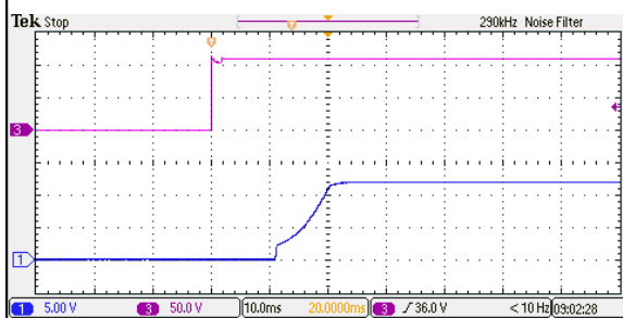
Figure 109: ERM01B110 Output Voltage Startup Characteristic by Vin Vin = 110Vdc Load: I_o = 1.67A Ch1: Vo Ch3: Vin
