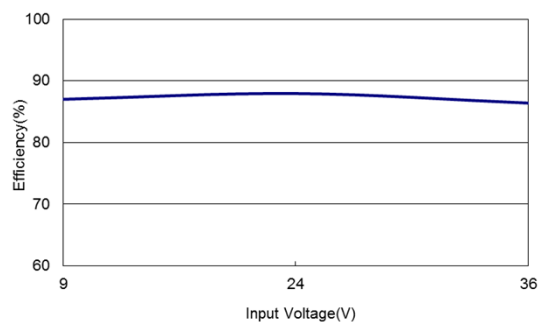
Figure 18: ERM01C18 Efficiency Versus Input Voltage Curve Vin = 9 to 36Vdc Load: Io = 1.33A
