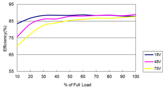
Figure 57: ERM01B36 Efficiency Versus Output Current Curve Vin = 18 to 75Vdc Load: Io = 0 to 1.67A
