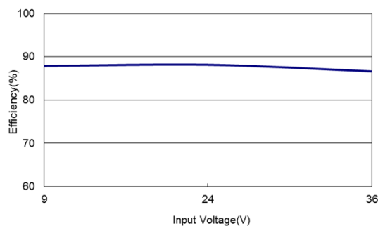
Figure 26: ERM01H18 Efficiency Versus Input Voltage Curve Vin = 9 to 36Vdc Load: Io = 0.833A
