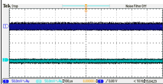
Figure 43: ERM01CC18 Ripple and Noise Measurement Vin = 24Vdc Load: Io = \pm 0.667A Ch 1: Vo1 Ch 2: Vo2
