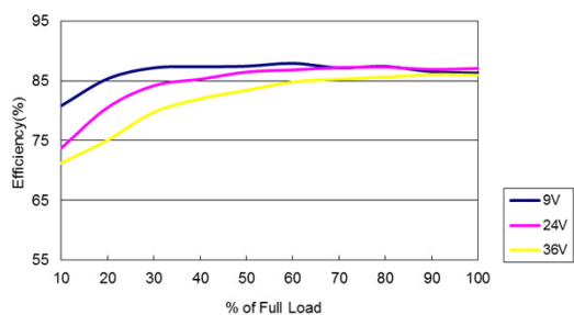
Figure 41: ERM01CC18 Efficiency Versus Output Current Curve Vin = 9 to 36Vdc Load: Io = 0 to \pm 0.667A
