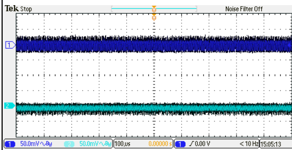
Figure 139: ERM01CC110 Ripple and Noise Measurement Vin = 110Vdc Load: Io = \pm 0.667A Ch 1: Vo1 Ch 2: Vo2
