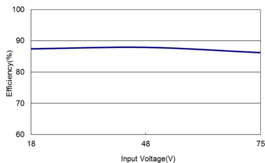
Figure 82: ERM01BB36 Efficiency Versus Input Voltage Curve Vin = 18 to 75Vdc Load: Io = \pm 0.833A
