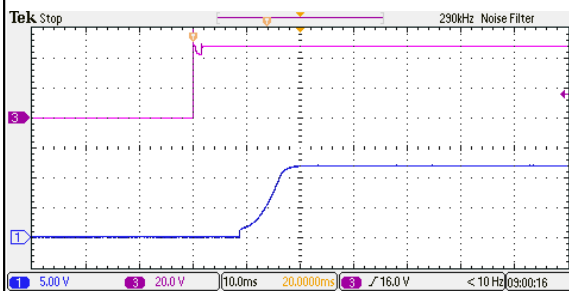
Figure 61: ERM01B36 Output Voltage Startup Characteristic by Vin Vin = 48Vdc Load: Io = 1.67A Ch1: Vo Ch3: Vin
