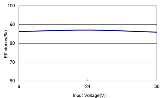
Figure 42: ERM01CC18 Efficiency Versus Input Voltage Curve Vin = 9 to 36Vdc Load: Io = \pm 0.667A
