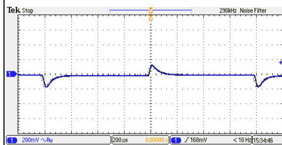
Figure 12: ERM01B18 Transient Response Vin = 24Vdc Load: I_o = 100\% to 75% load change Ch 1: Vo
