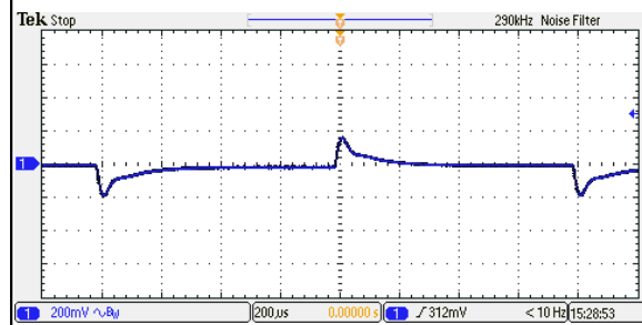
Figure 100: ERM04A110 Transient Response Vin = 110Vdc Load: Io = 100% to 75% load change Ch 1: Vo
