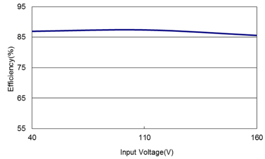
Figure 114: ERM01C110 Efficiency Versus Input Voltage Curve V_{in} = 40 to 160Vdc Load: I_o = 1.33A
