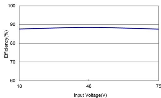
Figure 66: ERM01C36 Efficiency Versus Input Voltage Curve Vin = 18 to 75Vdc Load: Io = 1.33A
