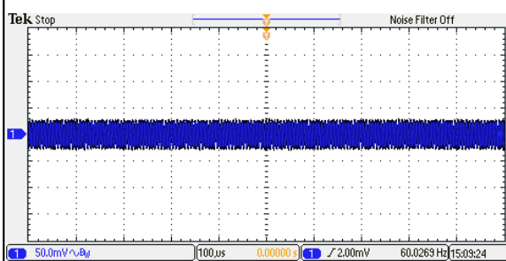
Figure 3: ERM04A18 Ripple and Noise Measurement Vin = 24Vdc Load: Io = 4A Ch 1: Vo
