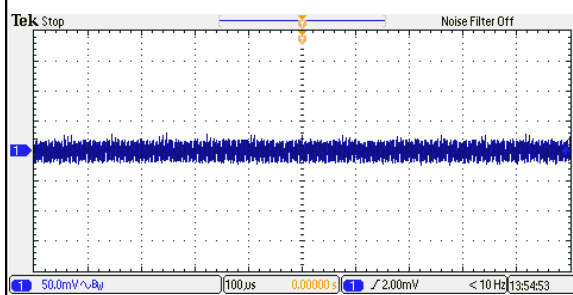
Figure 51: ERM04A36 Ripple and Noise Measurement Vin = 48Vdc Load: Io = 4A Ch 1: Vo
