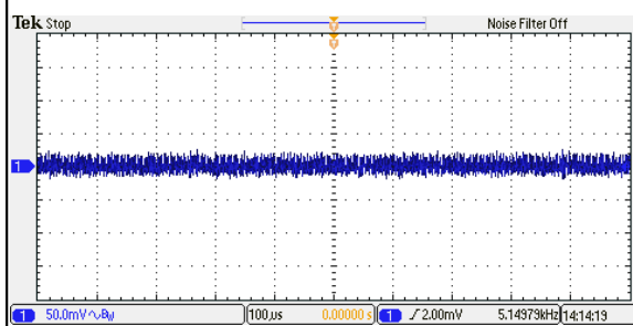
Figure 19: ERM01C18 Ripple and Noise Measurement Vin = 24Vdc Load: Io = 1.33A Ch 1: Vo
