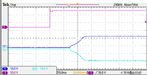
Figure 141: ERM01CC110 Output Voltage Startup Characteristic by Vin Vin = 110Vdc Load: Io = \pm 0.667A Ch1: Vo1 Ch2:Vo2 Ch3: Vin
