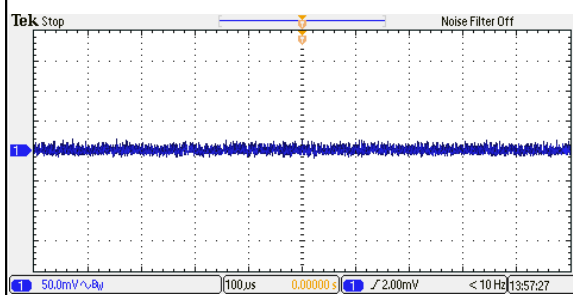
Figure 11: ERM01B18 Ripple and Noise Measurement Vin = 24Vdc Load: I_o = 1.67A Ch 1: Vo
