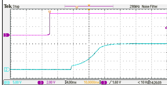
Figure 70: ERM01C36 Output Voltage Startup Characteristic by On/Off Vin = 48Vdc Load: Io = 1.33A Ch2: Vo Ch3: Vin
