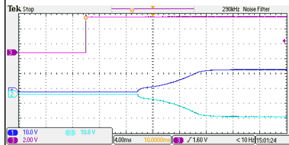
Figure 142: ERM01CC110 Output Voltage Startup Characteristic by On/Off Vin = 110Vdc Load: Io = \pm 0.667A Ch1: Vo1 Ch2:Vo2 Ch3: Vin
