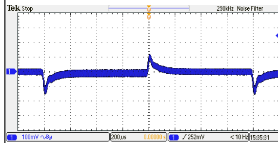
Figure 60: ERM01B36 Transient Response Vin = 48Vdc Load: Io = 100% to 75% load change Ch 1: Vo
