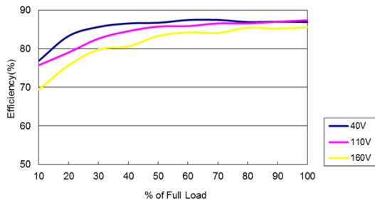
Figure 113: ERM01C110 Efficiency Versus Output Current Curve in = 40 to 160Vdc Load: I_o = 0 to 1.33A
