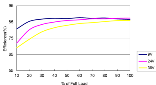
Figure 33: ERM01BB18 Efficiency Versus Output Current Curve Vin = 9 to 36Vdc Load: Io = 0 to \pm 0.833A
