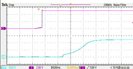
Figure 30: ERM01H18 Output Voltage Startup Characteristic by On/Off Vin = 24Vdc Load: Io = 0.833A Ch2: Vo Ch3: Vin
