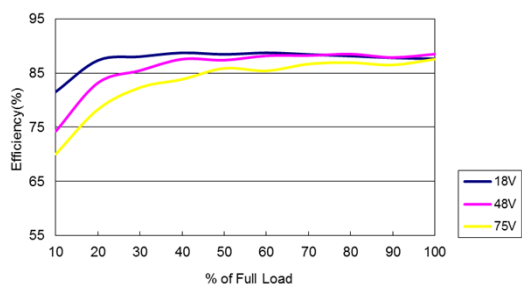
Figure 65: ERM01C36 Efficiency Versus Output Current Curve Vin = 18 to 75Vdc Load: Io = 0 to 1.33A
