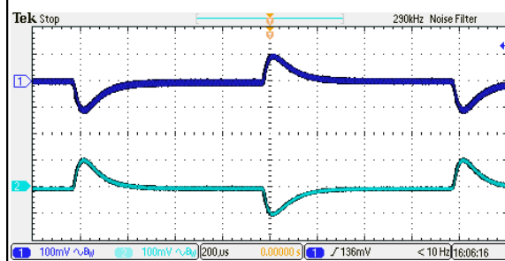
Figure 44: ERM01CC18 Transient Response Vin = 24Vdc Load: Io = 100% to 75% load change Ch 1: Vo1 Ch 2: Vo2
