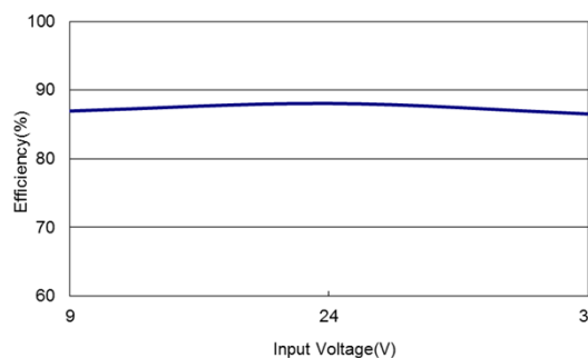
Figure 2: ERM04A18 Efficiency Versus Input Voltage Curve Vin = 9 to 36Vdc Load: Io = 4A
