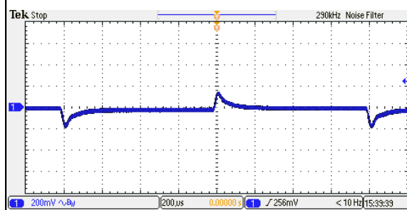
Figure 68: ERM01C36 Transient Response Vin = 48Vdc Load: Io = 100% to 75% load change Ch 1: Vo
