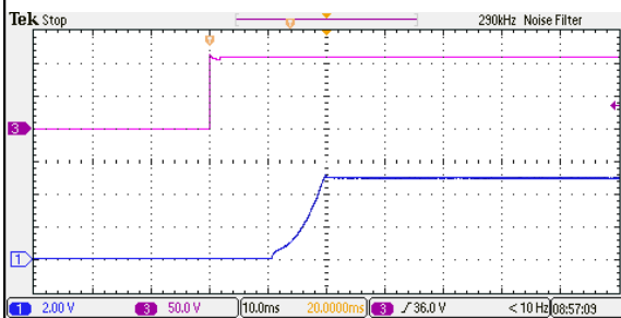
Figure 101: ERM04A110 Output Voltage Startup Characteristic by Vin Vin = 110Vdc Load: Io = 4A Ch1: Vo Ch3: Vin
