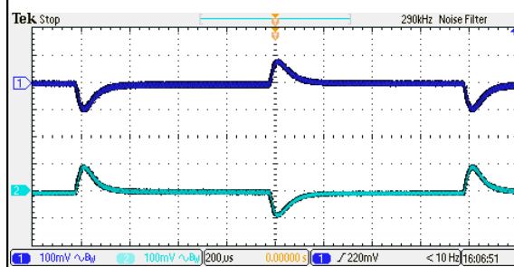
Figure 92: ERM01CC36 Transient Response Vin = 48Vdc Load: Io = 100% to 75% load change Ch 1: Vo1 Ch 2: Vo2
