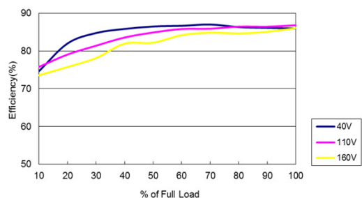
Figure 105: ERM01B110 Efficiency Versus Output Current Curve Vin = 40 to 160Vdc Load: I_o = 0 to 1.67A
