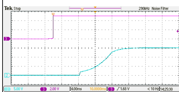
Figure 22: ERM01C18 Output Voltage Startup Characteristic by On/Off Vin = 24Vdc Load: Io = 1.33A Ch2: Vo Ch3: Vin
