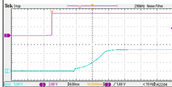
Figure 62: ERM01B36 Output Voltage Startup Characteristic by On/Off Vin = 48Vdc Load: Io = 1.67A Ch2: Vo Ch3: Vin
