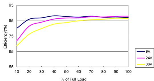
Figure 17: ERM01C18 Efficiency Versus Output Current Curve Vin = 9 to 36Vdc Load: Io = 0 to 1.33A
