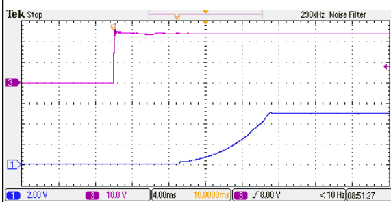
Figure 5: ERM04A18 Output Voltage Startup Characteristic by Vin Vin = 24Vdc Load: Io = 4A Ch1: Vin Ch3: Vo
