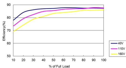
Figure 129: ERM01BB110 Efficiency Versus Output Current Curve Vin = 40 to 160Vdc Load: I_o = 0 to \pm 0.833A
