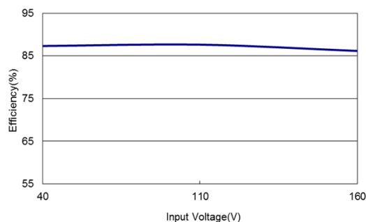
Figure 130: ERM01BB110 Efficiency Versus Input Voltage Curve Vin = 40 to 160Vdc Load: I_o = \pm 0.833A
