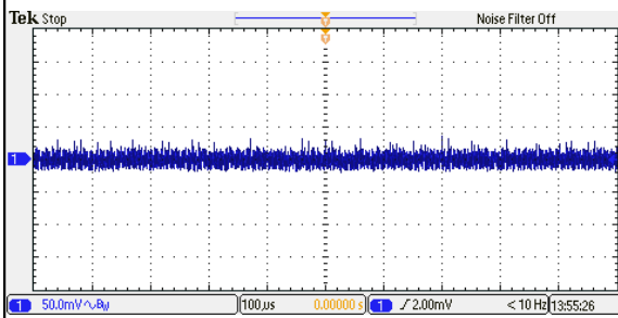
Figure 99: ERM04A110 Ripple and Noise Measurement Vin = 110Vdc Load: Io = 4A Ch 1: Vo
