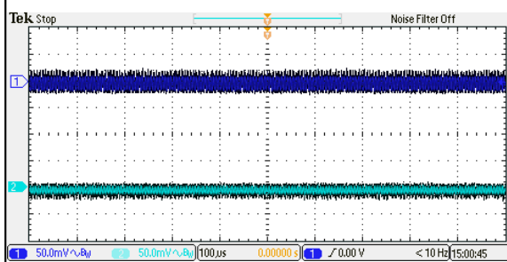
Figure 35: ERM01BB18 Ripple and Noise Measurement Vin = 24Vdc Load: Io = \pm 0.833A Ch 1: Vo1 Ch2: Vo2
