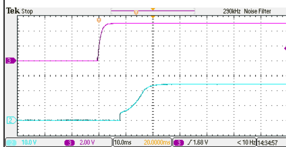
Figure 126: ERM01H36 Output Voltage Startup Characteristic by On/Off Vin = 110Vdc Load: Io = 0.833A Ch2: Vo Ch3: Vin
