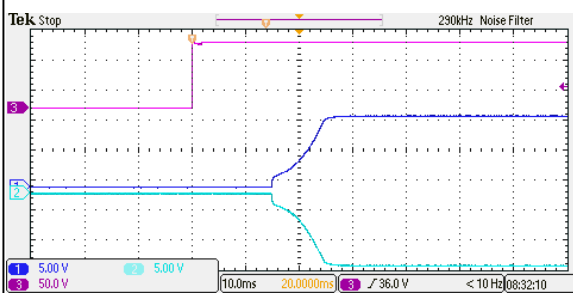
Figure 133: ERM01BB36 Output Voltage Startup Characteristic by Vin Vin = 110Vdc Load: I_o = \pm 0.833A Ch1: Vo1 Ch2: Vo2 Ch3: Vin
