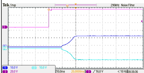
Figure 93: ERM01CC36 Output Voltage Startup Characteristic by Vin Vin = 48Vdc Load: Io = \pm 0.667A Ch1: Vo1 Ch2:Vo2 Ch3: Vin
