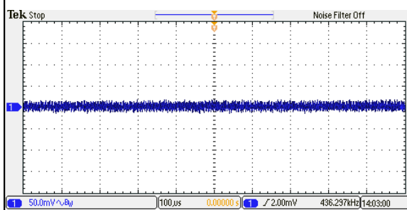
Figure 107: ERM01B110 Ripple and Noise Measurement Vin = 110Vdc Load: I_o = 1.67A Ch 1: Vo
