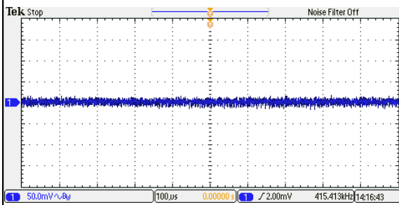
Figure 115: ERM01C110 Ripple and Noise Measurement V_{in} = 110Vdc Load: I_o = 1.33A Ch 1: V_o
