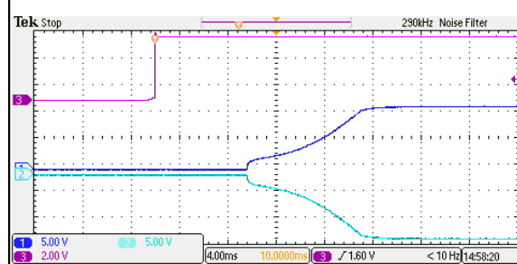
Figure 134: ERM01BB36 Output Voltage Startup Characteristic by On/Off Vin = 110Vdc Load: I_o = \pm 0.833A Ch1: Vo1 Ch2: Vo2 Ch3: Vin
