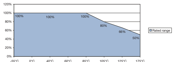
THJ 175°C Voltage vs Temperature Rating
