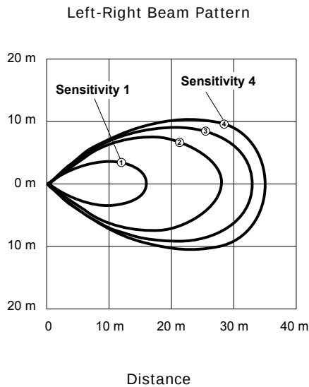
Typical Beam Pattern (with BRTR-CC20E Radar Target, Radar Cross Section = 50 \text{ m}^2 )
