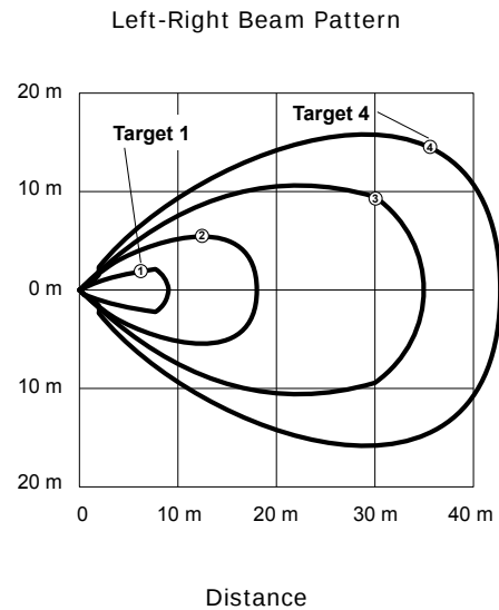
Typical Beam Pattern (with 4 different targets) at highest sensitivity level
