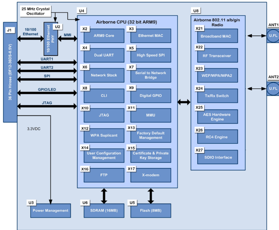
Figure 1 – APMN-Q551/WLNN-SE/SP/AN/ER-DP550 Family Block Diagram
