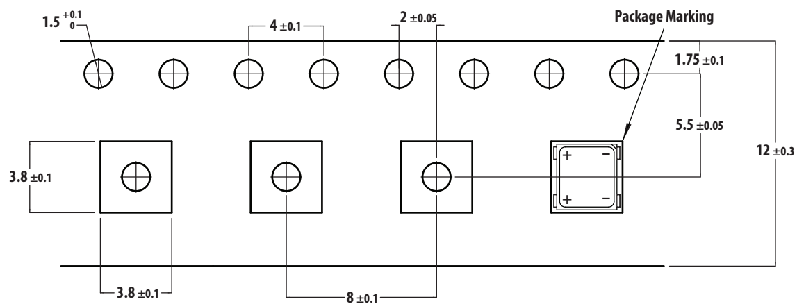
Figure 10. Carrier Tape Dimensions
