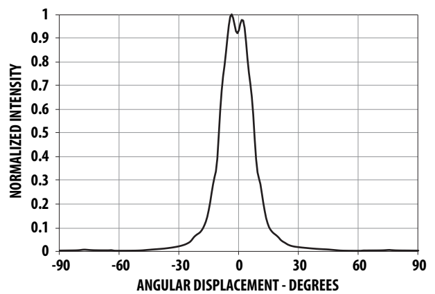
Figure 6. Representative Radiation pattern for 15° Viewing Angle Lamp
