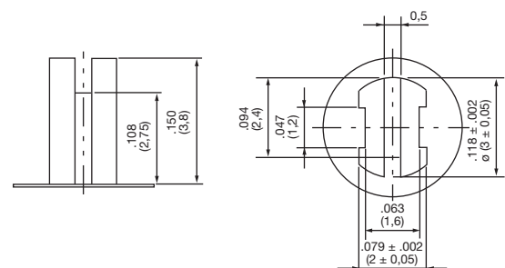
2 SHAFT FOR BUTTON
