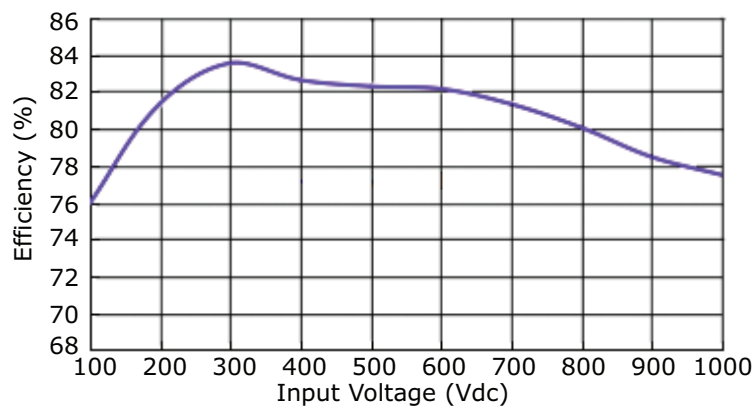
AE15-EW-S24 Efficiency Curve Efficiency vs. Input Voltage
