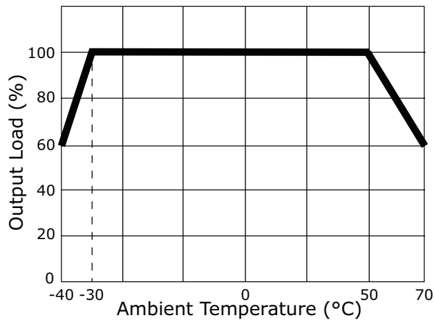
Temperature Derating Curve (100~150 Vdc input voltage)
