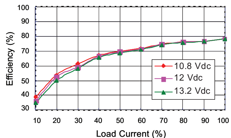
PCN1-S12-D5-M Efficiency Curve (Efficiency vs. Line Voltage and Load Current)
