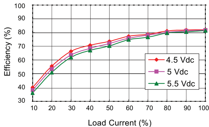
PCN1-S5-S12-M Efficiency Curve (Efficiency vs. Line Voltage and Load Current)
