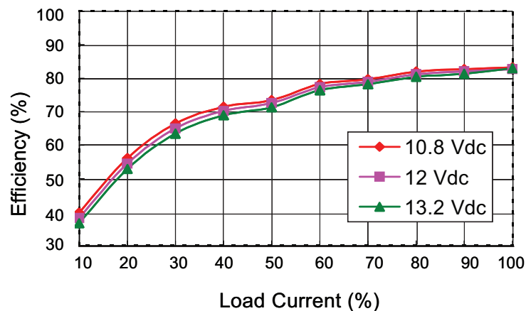
PCN1-S12-S12-M Efficiency Curve (Efficiency vs. Line Voltage and Load Current)
