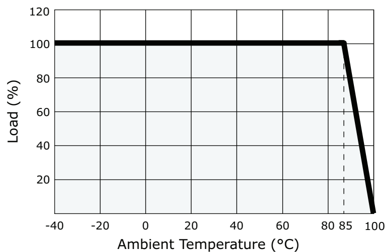
Temperature Derating Curve (Natural Convention)
