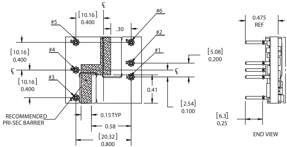
BOTTOM VIEW
