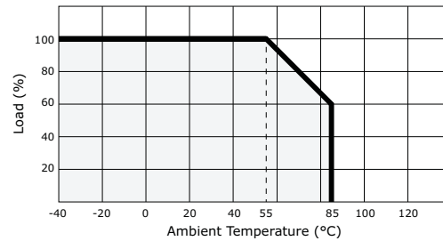
2. output power vs. ambient temperature ( \geq 5 V)
