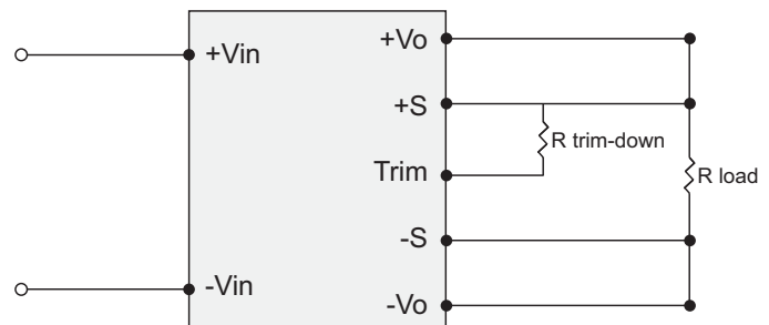
FIGURE 4: TRIM-DOWN VOLTAGE SETUP
